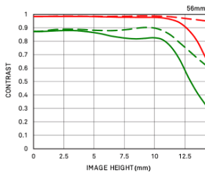
Geometrical MTF
