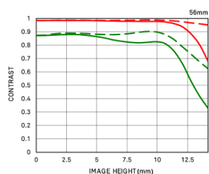
Geometrical MTF
