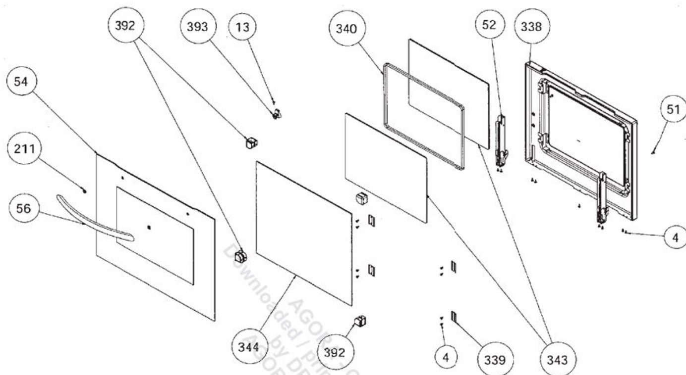
OVEN DOOR ASSEMBLY (OUTER & INNER) (POSITION NO 378)
