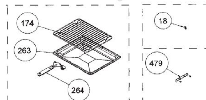
TRAY SET FOR GRID ( POSITION NO 265 ) (OPTIONAL)
