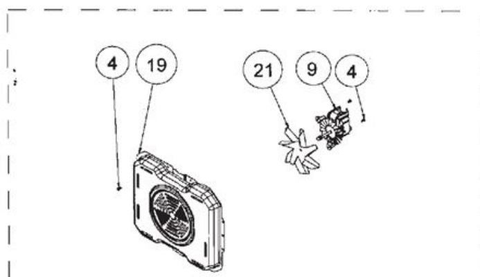
(FAN COVER/FAN IMPELLER (6 WINGS )/FAN MOTOR) (OPTIONAL)
