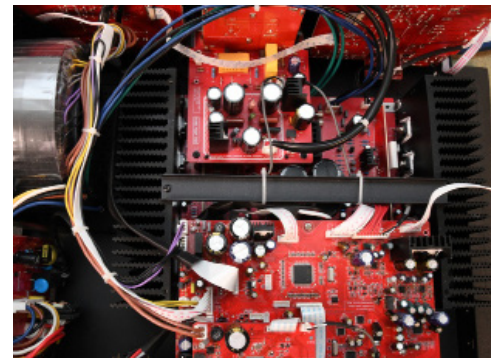
Independence of the right and left channel in terms of cooling and power transistors.
