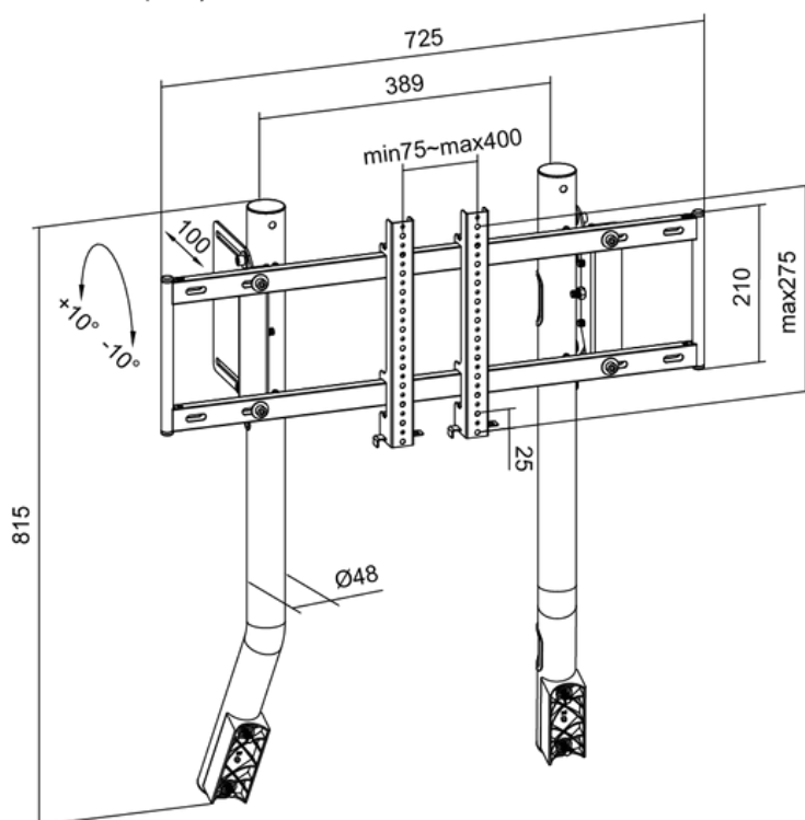
Dimensions (mm)
