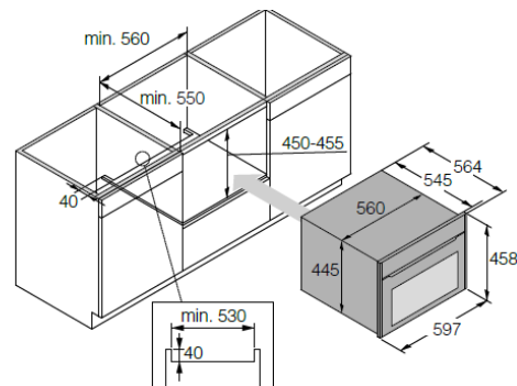
Under-counter installation
