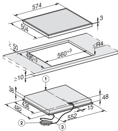
KM 6527 FR (Installation drawing)
