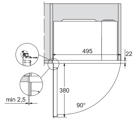
M2224SC, installation drawing
