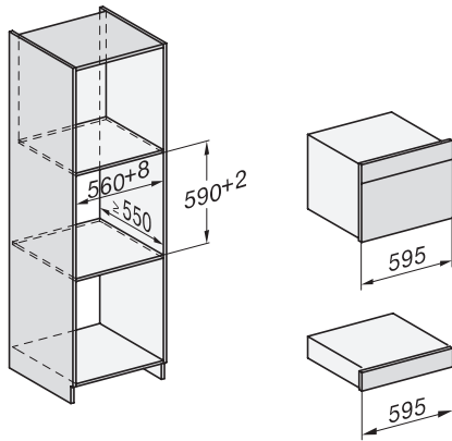
ESW7x10, DGC7x4xHCPPro, DGC7x4xHCXPro, installation drawings
