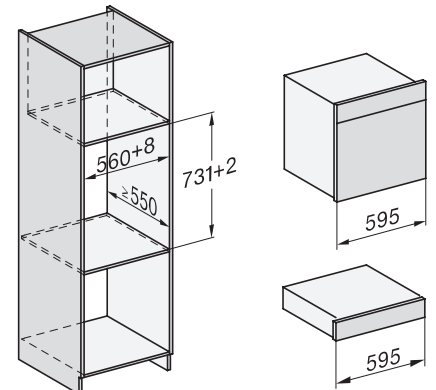
ESW7x10, EVS7010, DGC7x6xHCPPro, DGC7x6xHCXPro installation drawings
