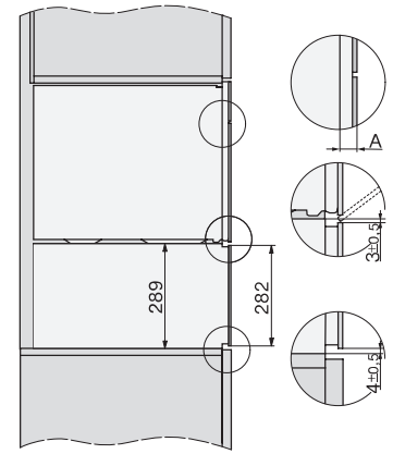
ESW7x20, DG7xxx, DGM7xxx installation drawings
