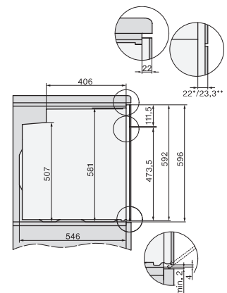
side view H7000 XL build-under, installation drawing
