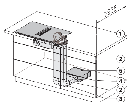
KMDA7272-1FL/FR, KMDA7473-1FL/FR, KMDA7272FL/FR, KMDA7473FL/FR – Installation variant 3 Basis
