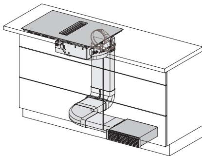
KMDA7272-1FL/FR, KMDA7272FL/FR – Operating options
