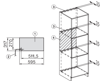
ESW7030 installation drawings
