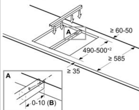
measurements in mm Assembly kit (HEZ394301) for Domino
