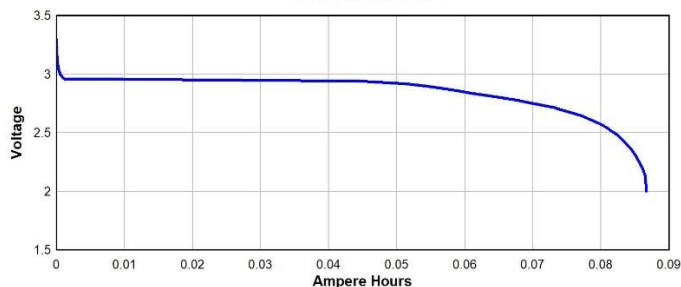
IEC Rated Capacity 30K Ohm Continuous to 2V
