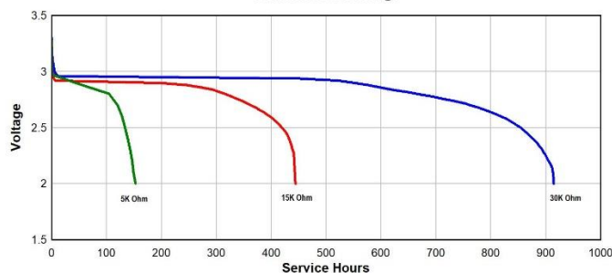
Continuous Discharge
