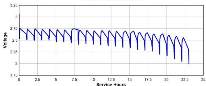
Pulse Discharge 270 Ohm / 1300 Ohm, 5m/h to 2V
