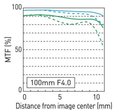
MTF Chart — 20S — 20M — 40S — 40M
