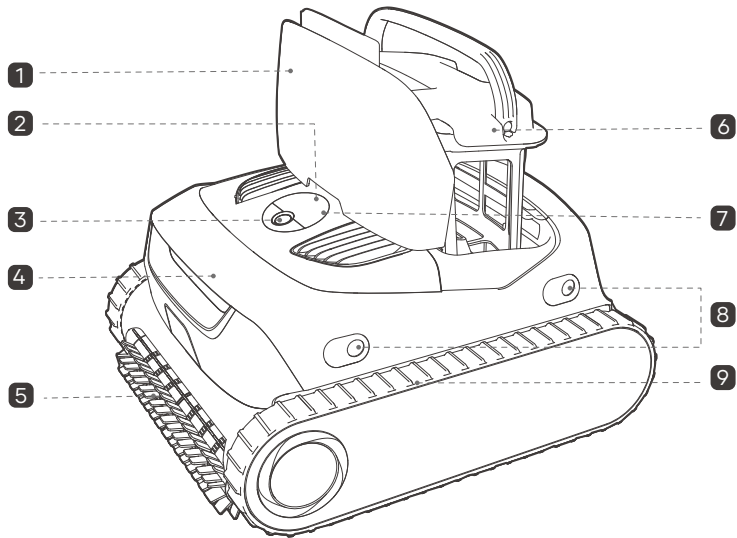
Robotic Pool Cleaner (Side View)
