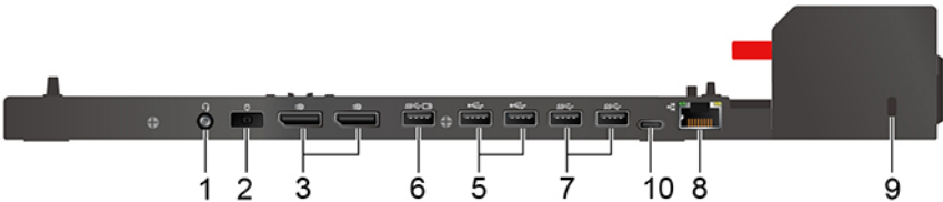
Figure 2. ThinkPad Pro Docking Station
