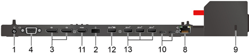
Figure 3. ThinkPad Ultra Docking Station
