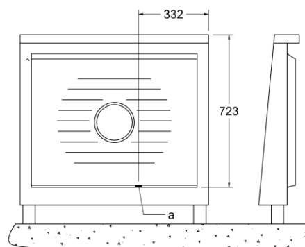
CONNECTION DETAILS
