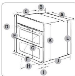
Oven (mm)
